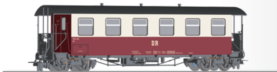
Schmalspur-Personenwagen KB4ip der DR Narrow gauge passenger coach KB4ip of the DR
